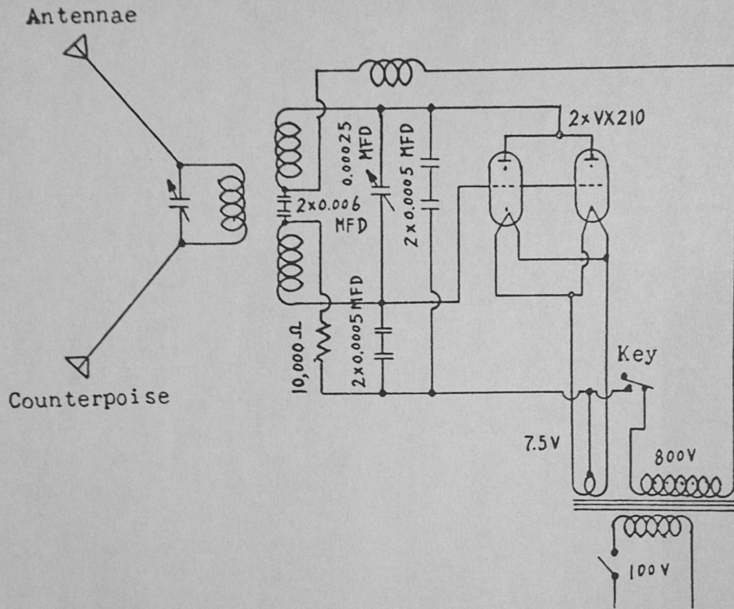
Circuit Diagram of Max Klausen's Radio Transmitter
