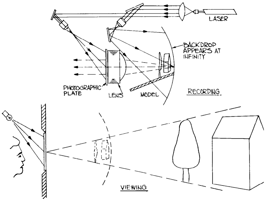
Fig. 31. Panoramic Holography.
